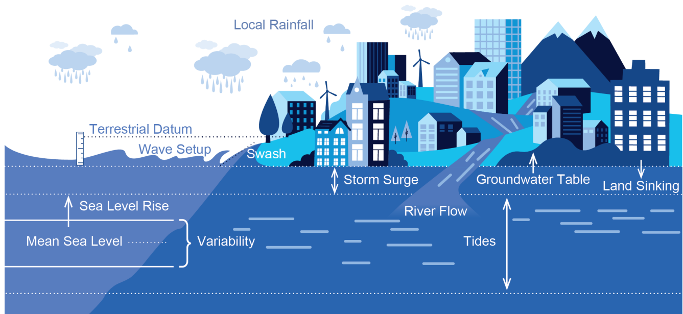
Figure 1.1: Schematic (not to scale) showing physical factors affecting coastal flood exposure. Due to the clear and strong relative sea level rise signal (i.e., combination of sea level rise and sinking lands), the probability of flooding and impacts are increasing along most U.S. coastlines.
