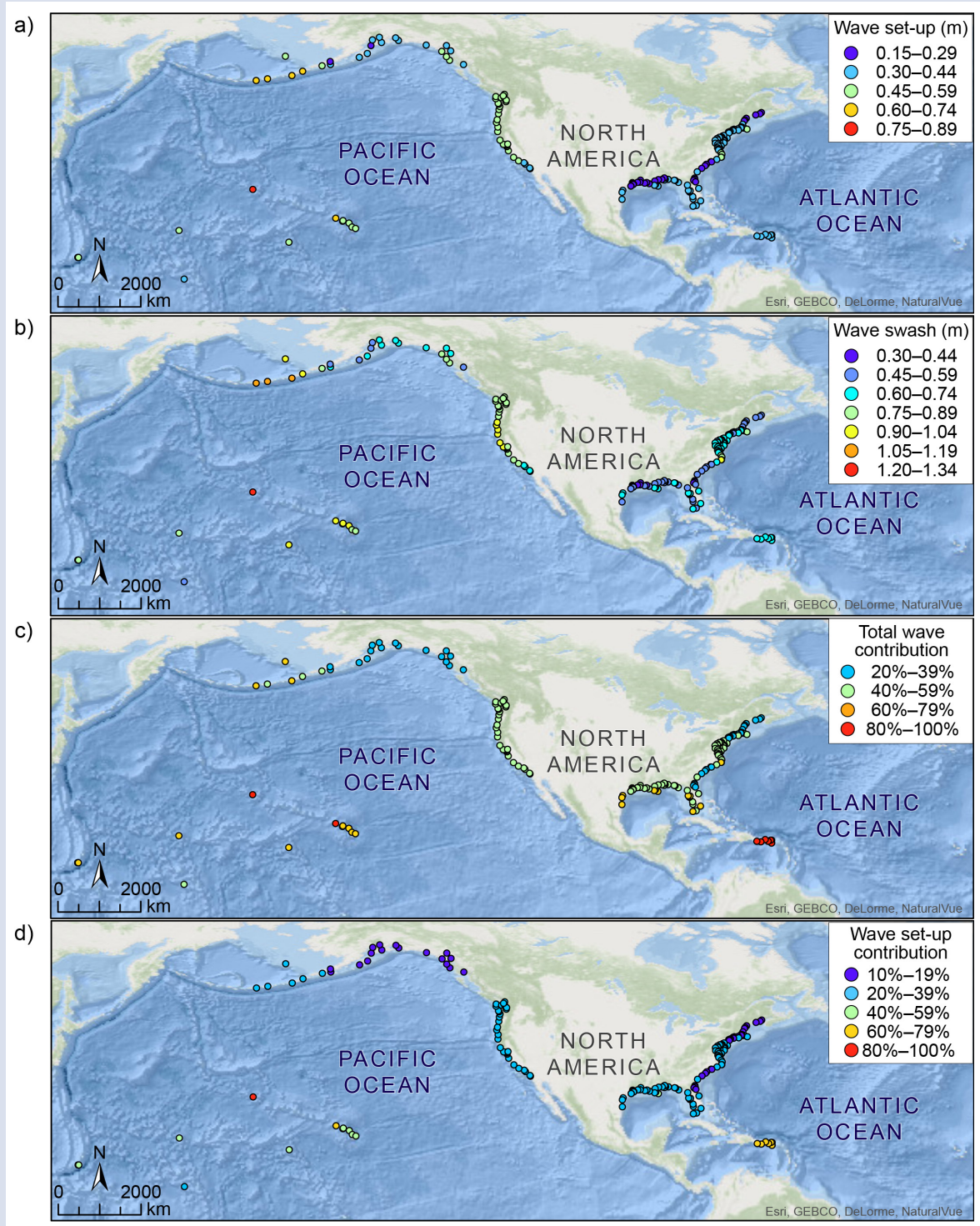
Figure Box 3.1. Water level contribution due to a) wave set-up and b) wave wash; c) percent contribution of wave-driven water levels (i.e., wave run up = wave set-up and wash) relative to all components: tide, storm surge, and waves; and d) percent contribution of wave set-up relative to the sum of tide, storm surge, and wave set-up based on model reanalysis of Vitousek et al. (2017).
