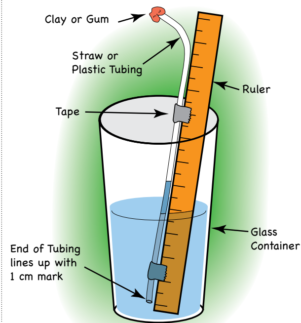
Figure 3. Barometer
